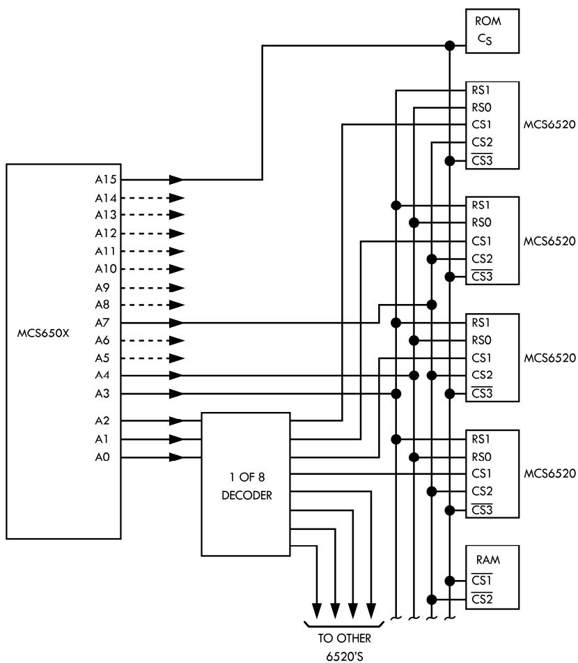
Page Zero Chip Select Addressing Scheme FIGURE 2.11
