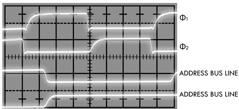
Proper Address Lines
