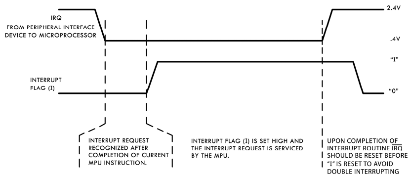
Sequence to Service \overline{IRQ} FIGURE 1.10
